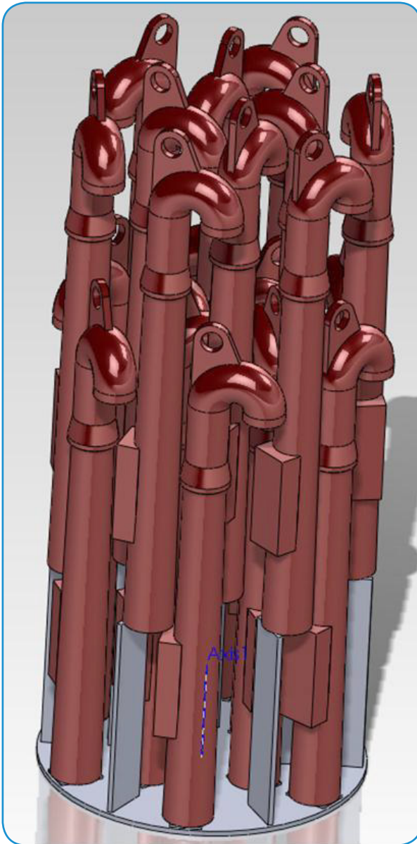
Jet Pump RWC layout
