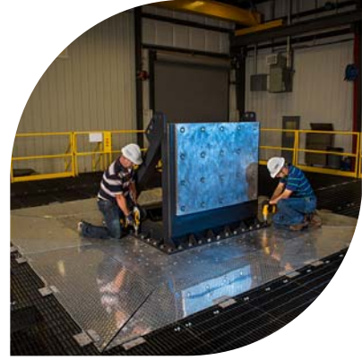
The Shake Table with 10,000 lbs. during testing
