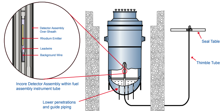
Fixed In-core Detector System utilizing existing vessel penetrations and thimble tube in a Westinghouse-Type reactor, requiring no facility modifications.
