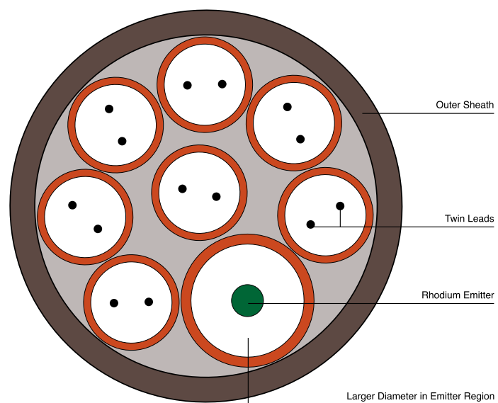
Advanced Twin-Lead In-core Detector Assembly (For higher accuracy; longer life)
